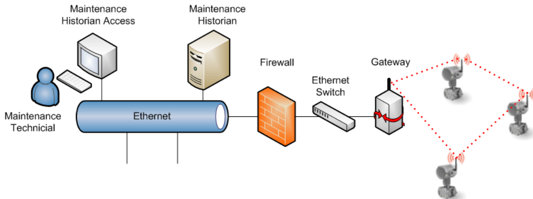
Figure 16. Gateway Integration Into Host System
